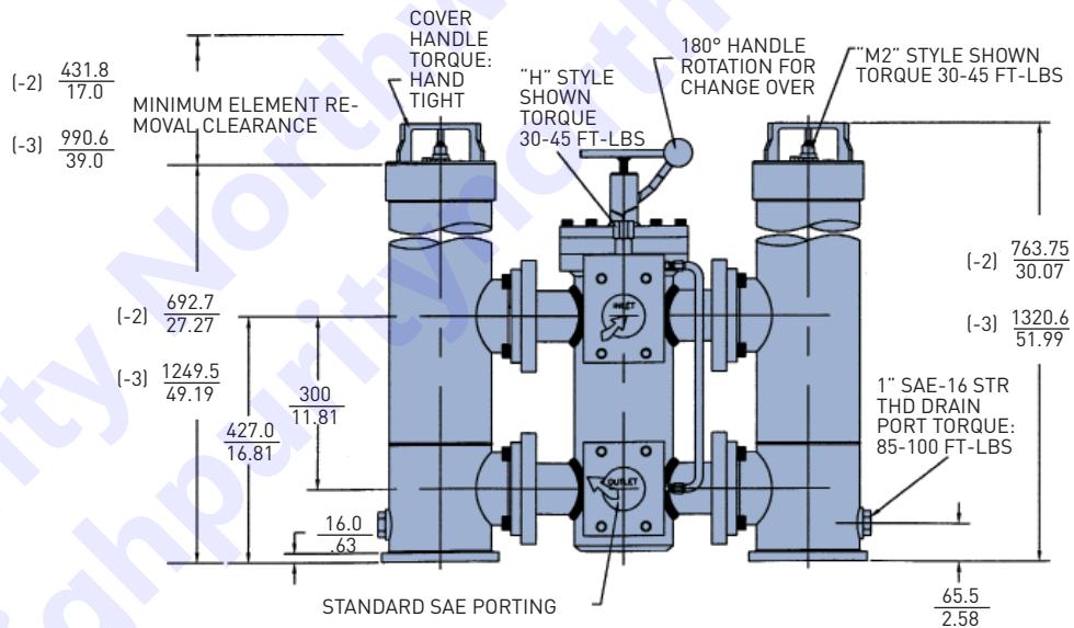
HDIL8/HQIL8 Side View
