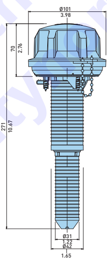
Telescopic Strainer
