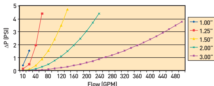
Flow Vs. Pressure Loss
