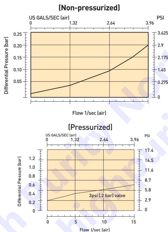
Telescopic Strainer
